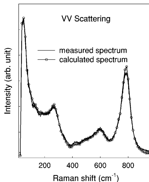
FIG. 7. Calculated Raman spectra in comparison with the observed Raman spectra of the PZN-8%PT crystal at one arbitrary intermediate electric field of 27.3 kV/cm in the parallel (VV) scattering geometry. Details of calculation are in the text.
