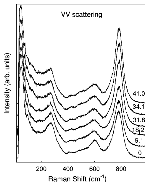
FIG. 2. Room-temperature (22.5 °C) Raman spectra of the PZN-8%PT crystal at various electric fields (kV/cm) applied in the (001) direction in the parallel (VV) scattering geometry. Each spectrum is shifted by constant amount in intensity for clarity.
