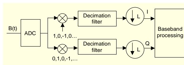
Fig. 2. Simplified DDC architecture.
